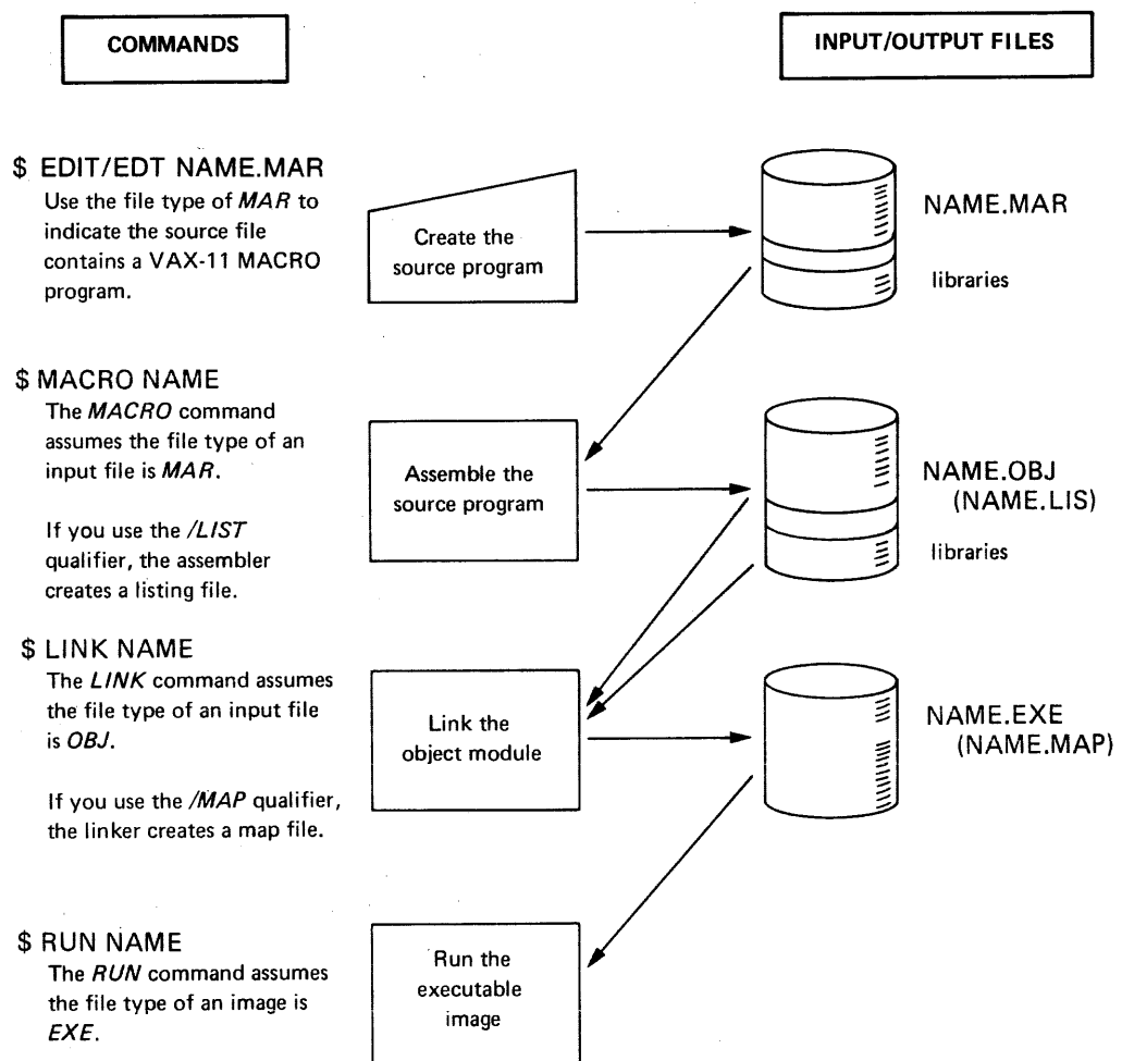
Figure 4-3: Commands for MACRO Program Development
